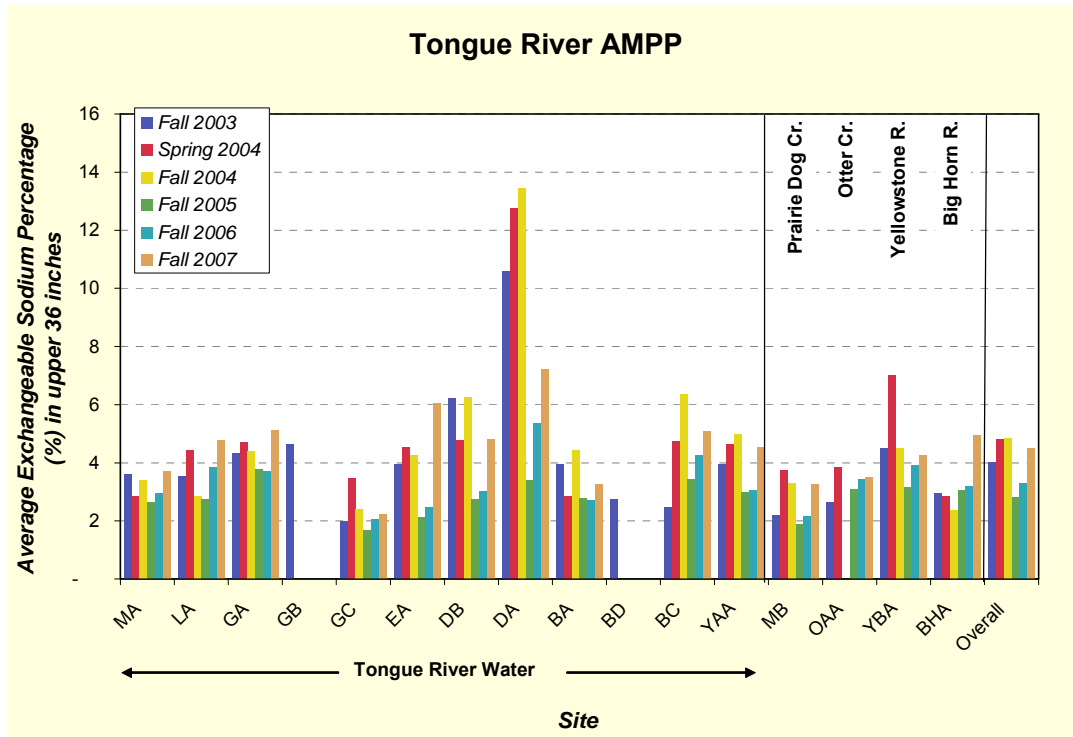
Figure L. Average ESP (percent) to 36 inches in AMPP sites for each sampling period.
